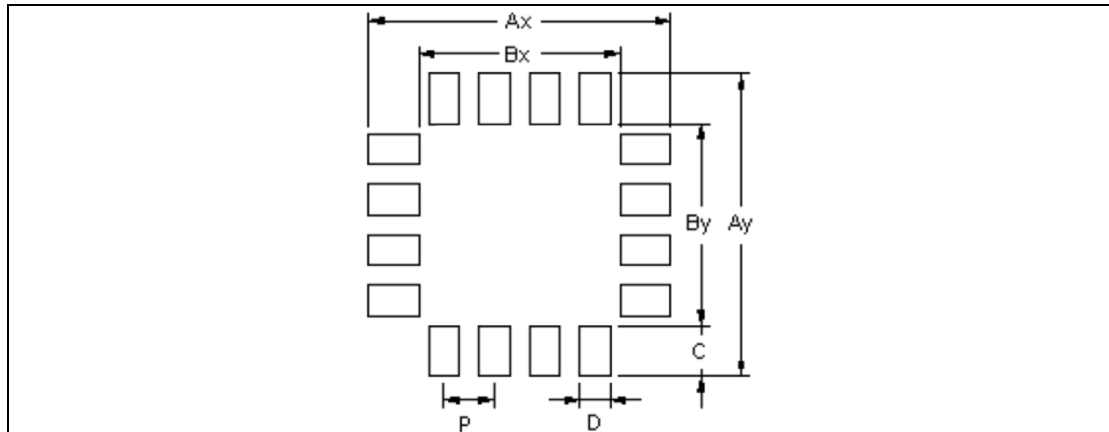
Figure 18: QFN16 footprint: Please refer to the Table 12 for the dimensions. For best temperature accuracy it is not recommended to solder the thermal pad of the QFN package to the printed circuit board
