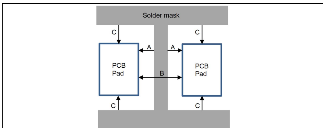
Figure 19: If necessary, the edge of the solder mask opening around the PCB pads can be set up to the edge of the pad (A). If the distance between the pads is insufficient for the solder mask (B) then the mask can be set to the bottom and the top edges of the pads (C).
