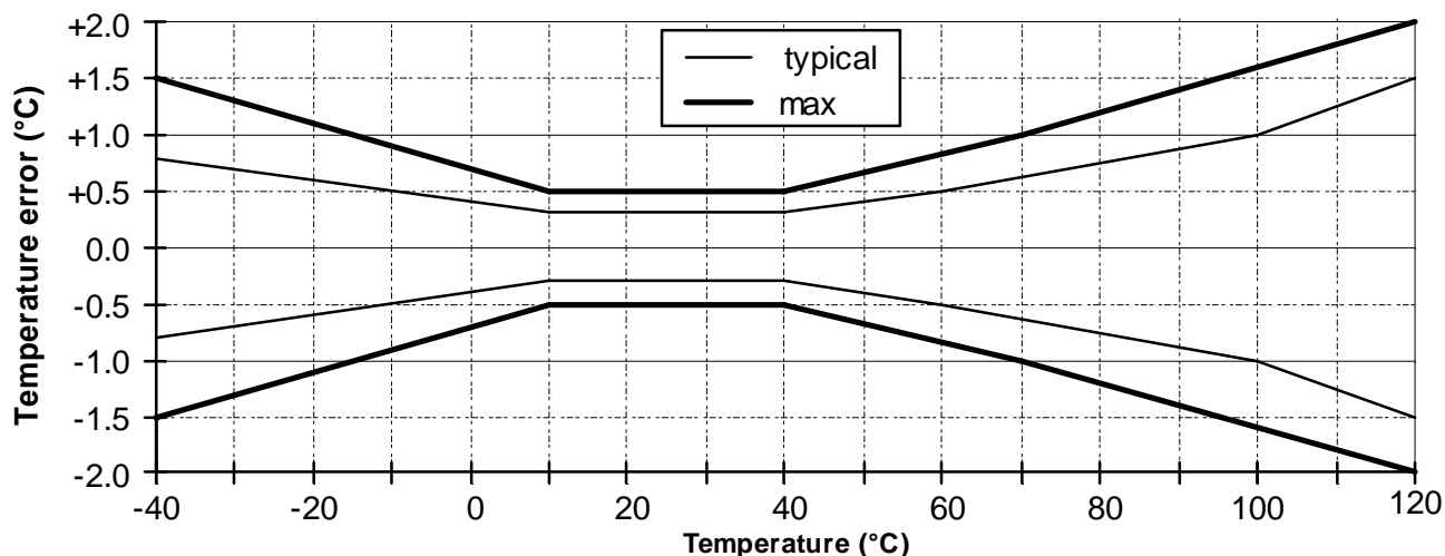
Figure 13: Temperature accuracy
